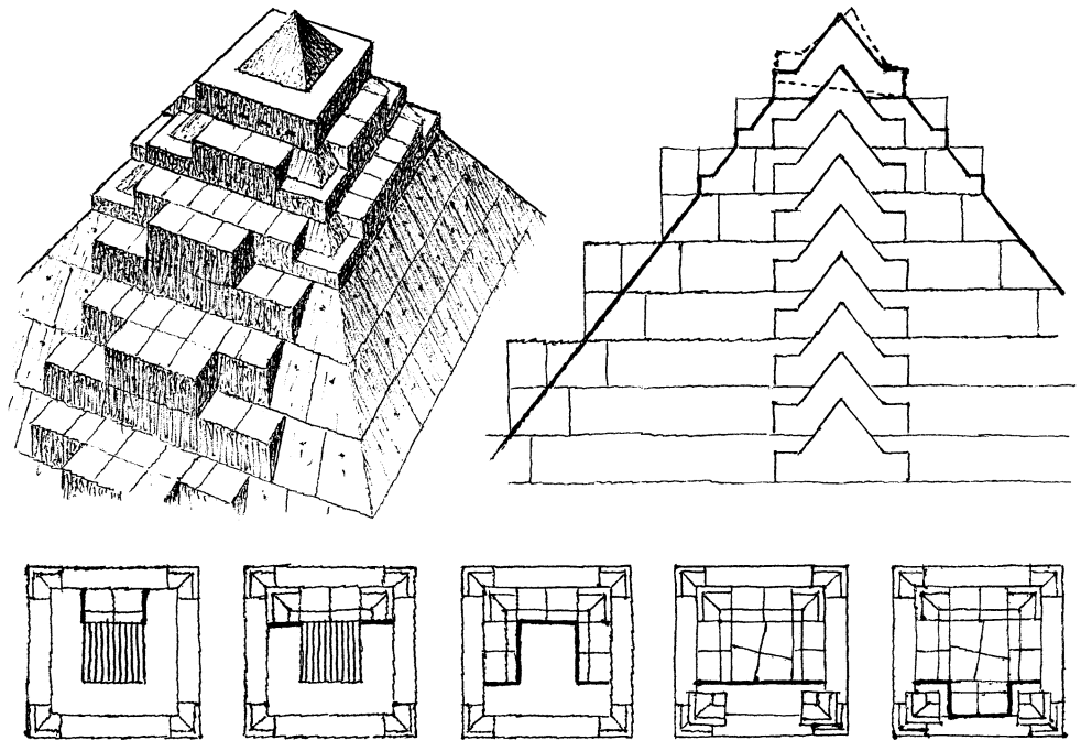
Fig. 5. Schematic diagram (right) of incremental lifts of the capstone block. Bird's-eye view (left) of top of pyramid, showing access stairway and constructional ledges at the two uppermost courses. Series of plan views (below) indicating the order of installation for all the blocks in the highest course, just below the capstone. Core blocks beneath the capstone would have had slightly skewed joints (exaggerated in the drawing) to permit their snug installation.
